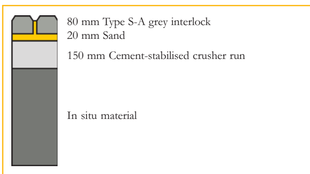
Figure 13: Pavement design - Bellville Goods Yard.
