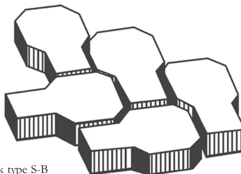
Figure 3b: Type S-B: Those blocks which allow geometrical interlock between some faces of adjacent blocks.
