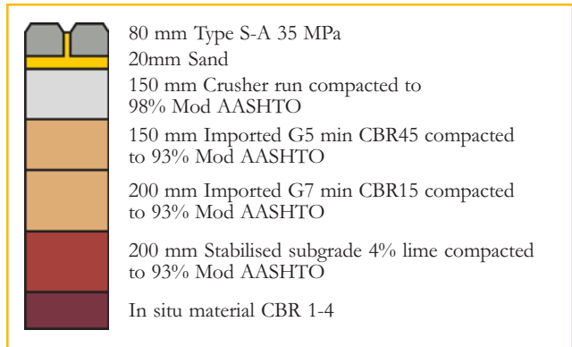
Figure 14: Pavement design Trident steel.
